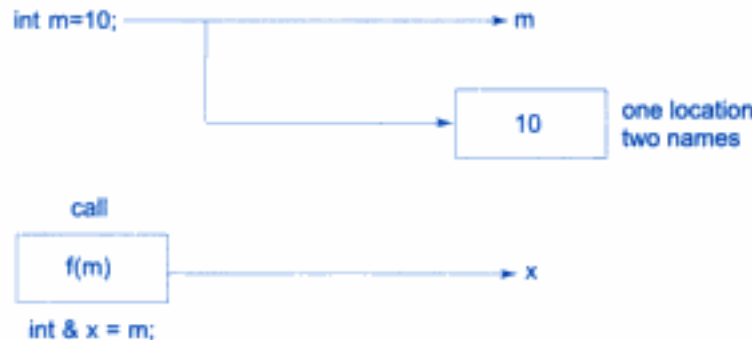
Fig. 3.2 \Rightarrow Call by reference mechanism
