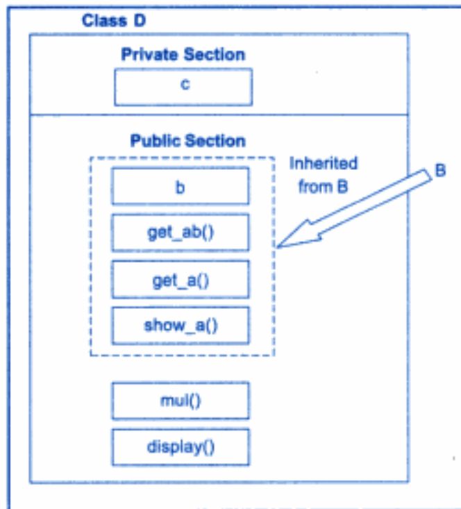
Fig. 8.2 \Leftrightarrow Adding more members to a class (by public derivation)
