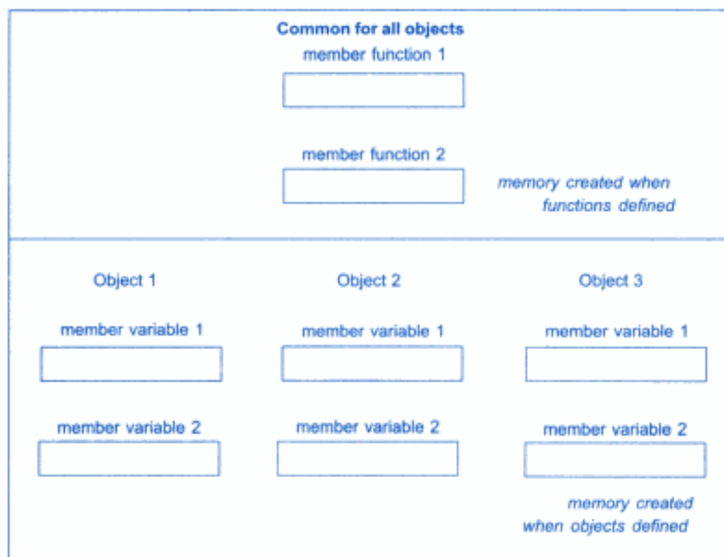
Fig. 5.3 ⇔ Object of memory
