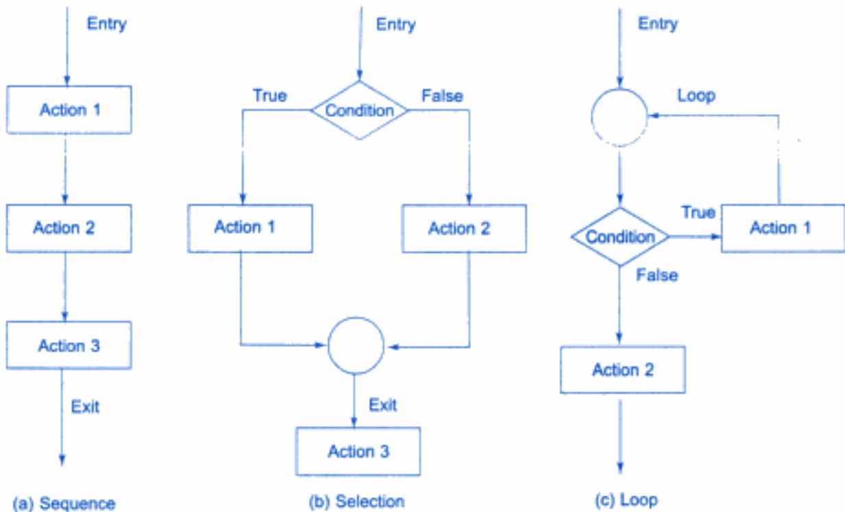
Fig. 3.4 ⇔ Basic control structures
