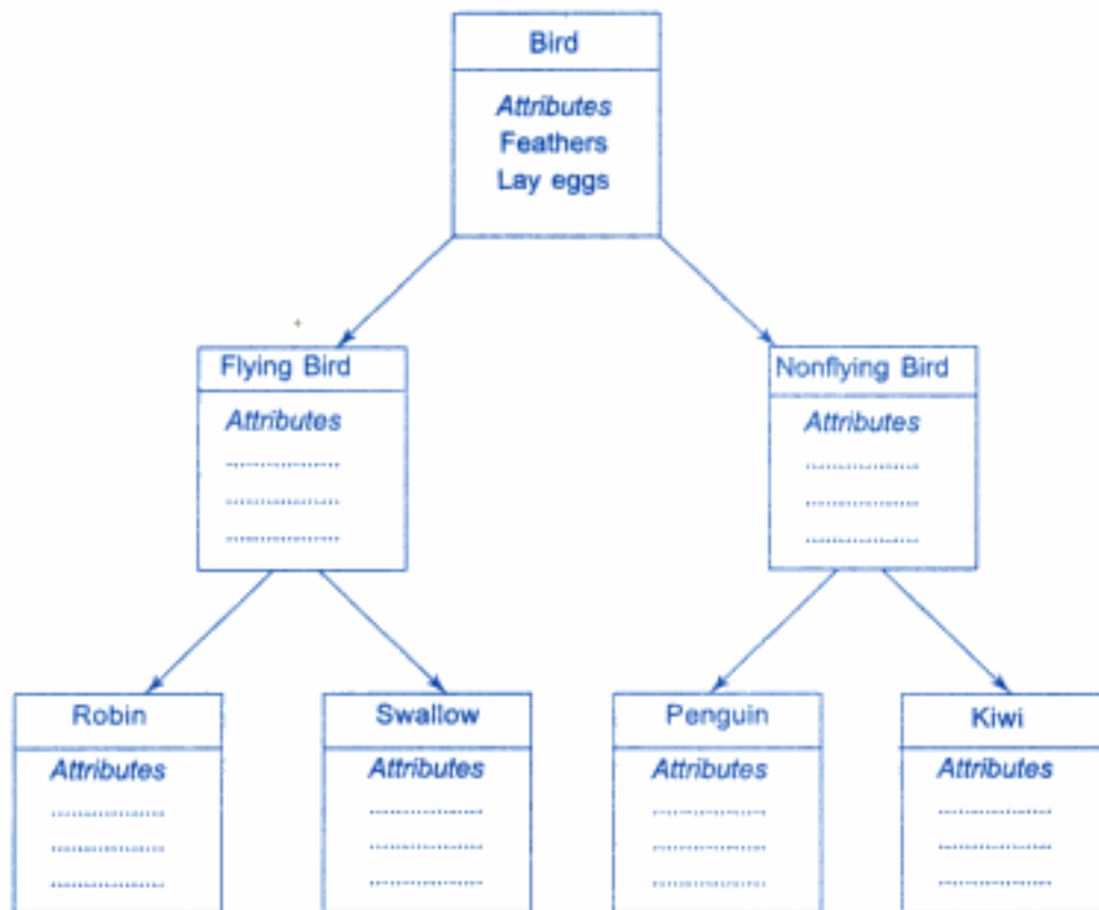
Fig. 1.8 \Leftarrow Property inheritance
