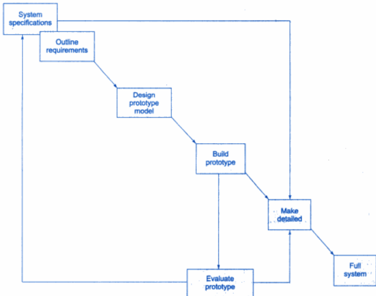
Fig. 17.22 ⇔ Prototype paradigm
