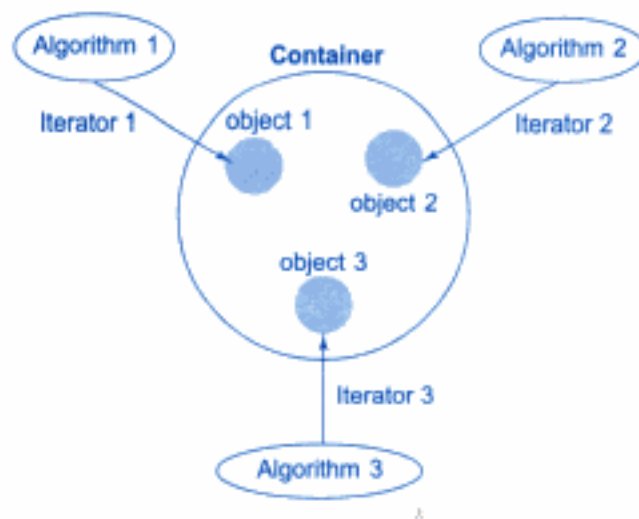
Fig. 14.1 ⇔ Relationship between the three STL components
