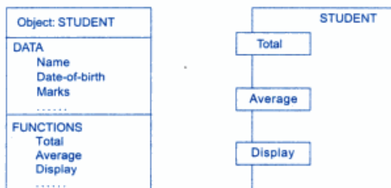
Fig. 1.7 \Rightarrow Two ways of representing an object
