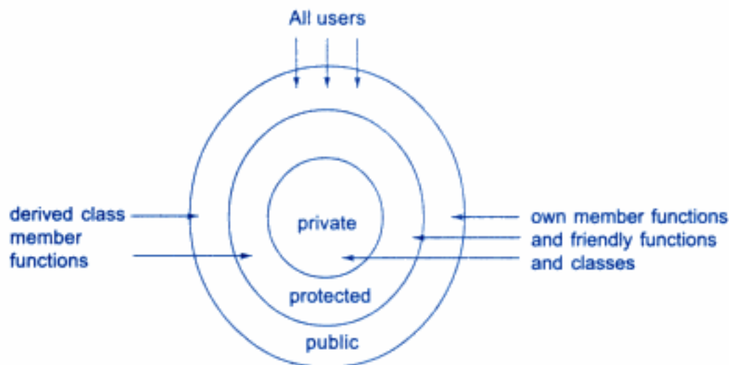
Fig. 8.6 \Leftrightarrow A simple view of access control to the members of a class
