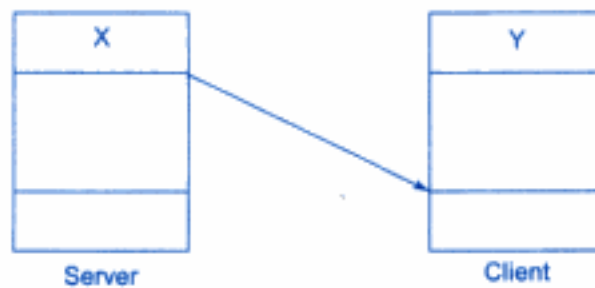
Fig. 17.13 ⇔ Client-server relationship
