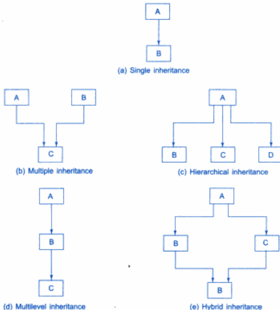
Fig. 8.1 ⇔ Forms of inheritance
