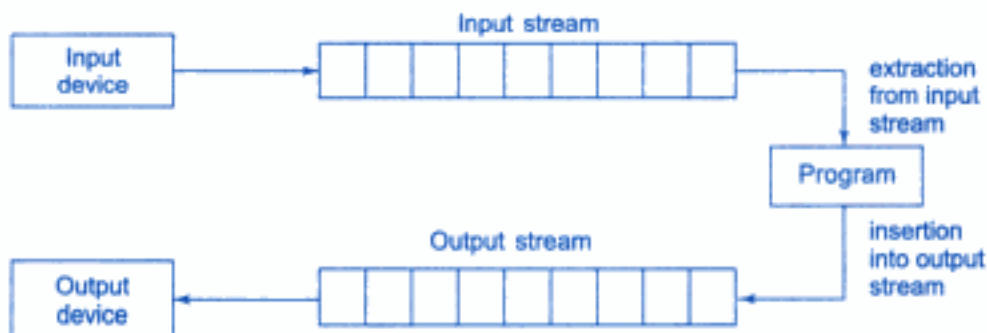
Fig. 10.1 ⇔ Data streams
